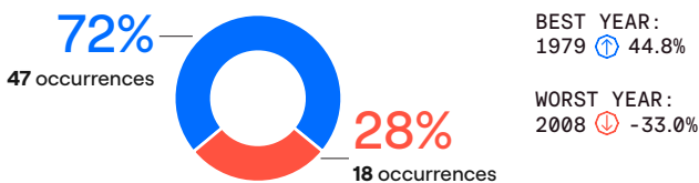
Figure 4: 3-year rate of return for all-equity vs. balanced portfolio
